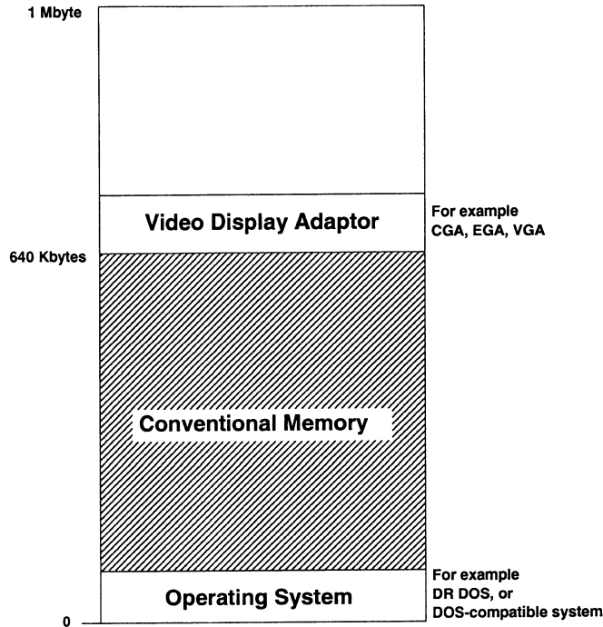
Figure C.1 8086 Memory Map
